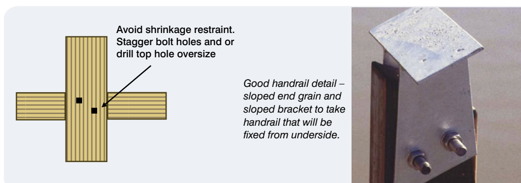
Figure 6.6: Good detailing.
