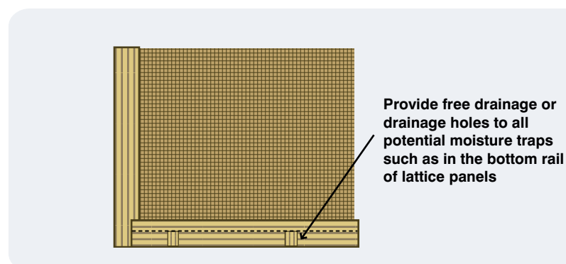
Figure 6.5: Drainage holes.
